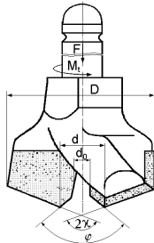
Fig. 1. Detachable bit
